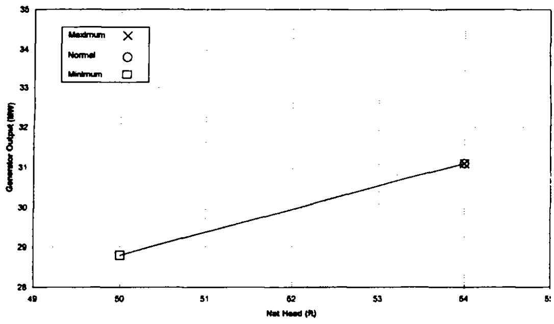
Falls Plant Capability Curve Existing Units
