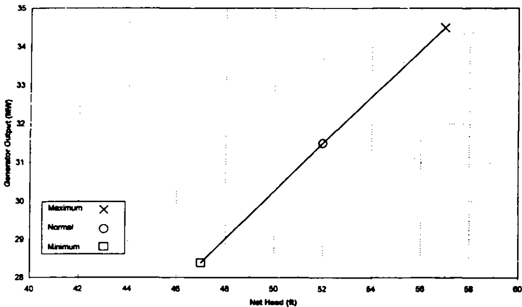
High Rock Plant Capability Curve Existing Units
