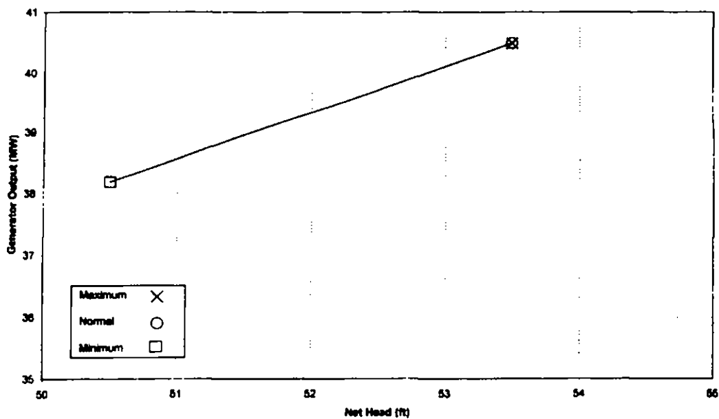
Tuckertown Plant Capability Curve Existing Units
