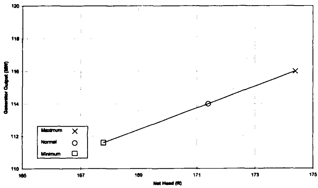
Narrows Plant Capability Curve Existing Units
